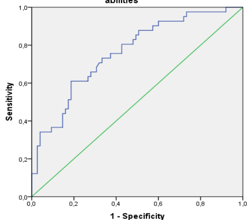
ROC curves with predicted values from logistic regression model of functional abilities
